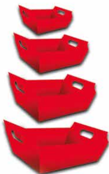
REF. 06
